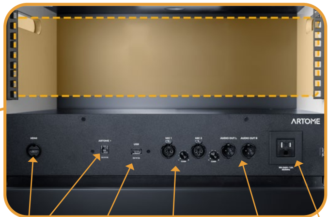
HDMI & USB-B USB-A (5V=1A) Mic 1 & 2 XLR (Mic or Line in option) Audio Out XLR Power Outlet
