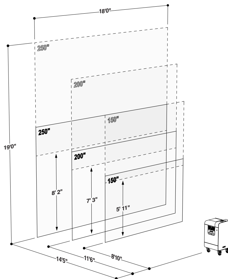
Example of projection distances with the Panasonic PT-VMZ7ST projector
